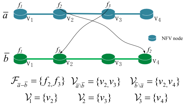
Fig. 2. Illustration of the definitions of \mathcal{F}_{\bar{a}-\bar{b}} , \mathcal{V}_{\bar{a}\bar{b}} , and \mathcal{V}_{\bar{b}\bar{a}} .
