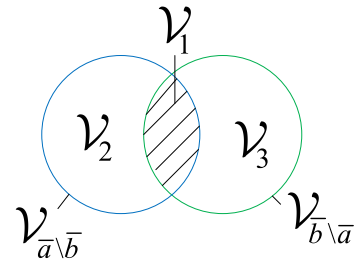
Fig. 3. Illustration of the relationships between the sets \mathcal{V}_{\bar{a}\bar{b}} , \mathcal{V}_{\bar{b}\bar{a}} , \mathcal{V}_1 , \mathcal{V}_2 , and \mathcal{V}_3 .
